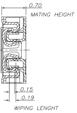
MATED CROSS SCALE 2:1
